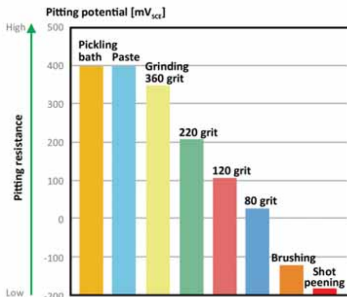
Figure 2: The graph shows how pickling gives the best pitting resistance when compared to grit grinding and other surface cleaning techniques (graph courtesy Outokumpu).
