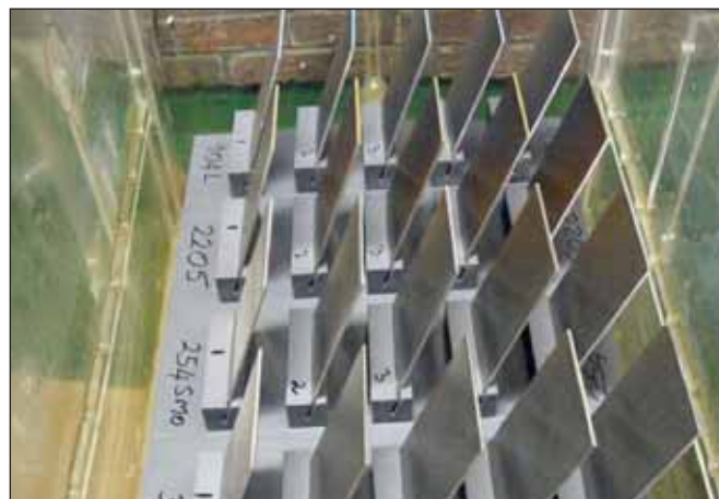
Figure 3: Accelerated corrosion testing of various stainless steels to prove capability in a selected corrosive atmosphere – in this case Calcium chloride and Acetic acid at 75°C.
