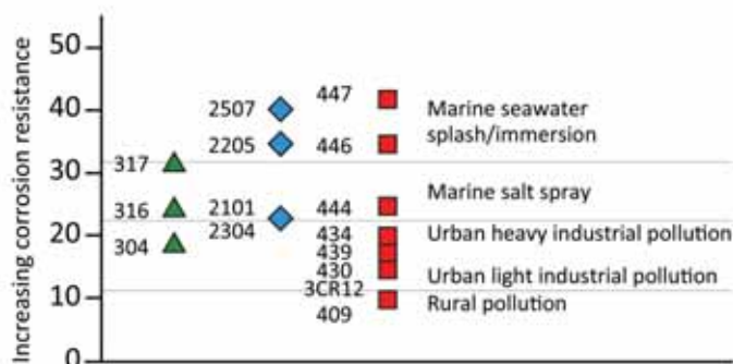
Figure 1.2: Relative corrosion performance of selected stainless steels.
